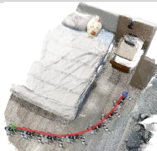
StreamVLN
